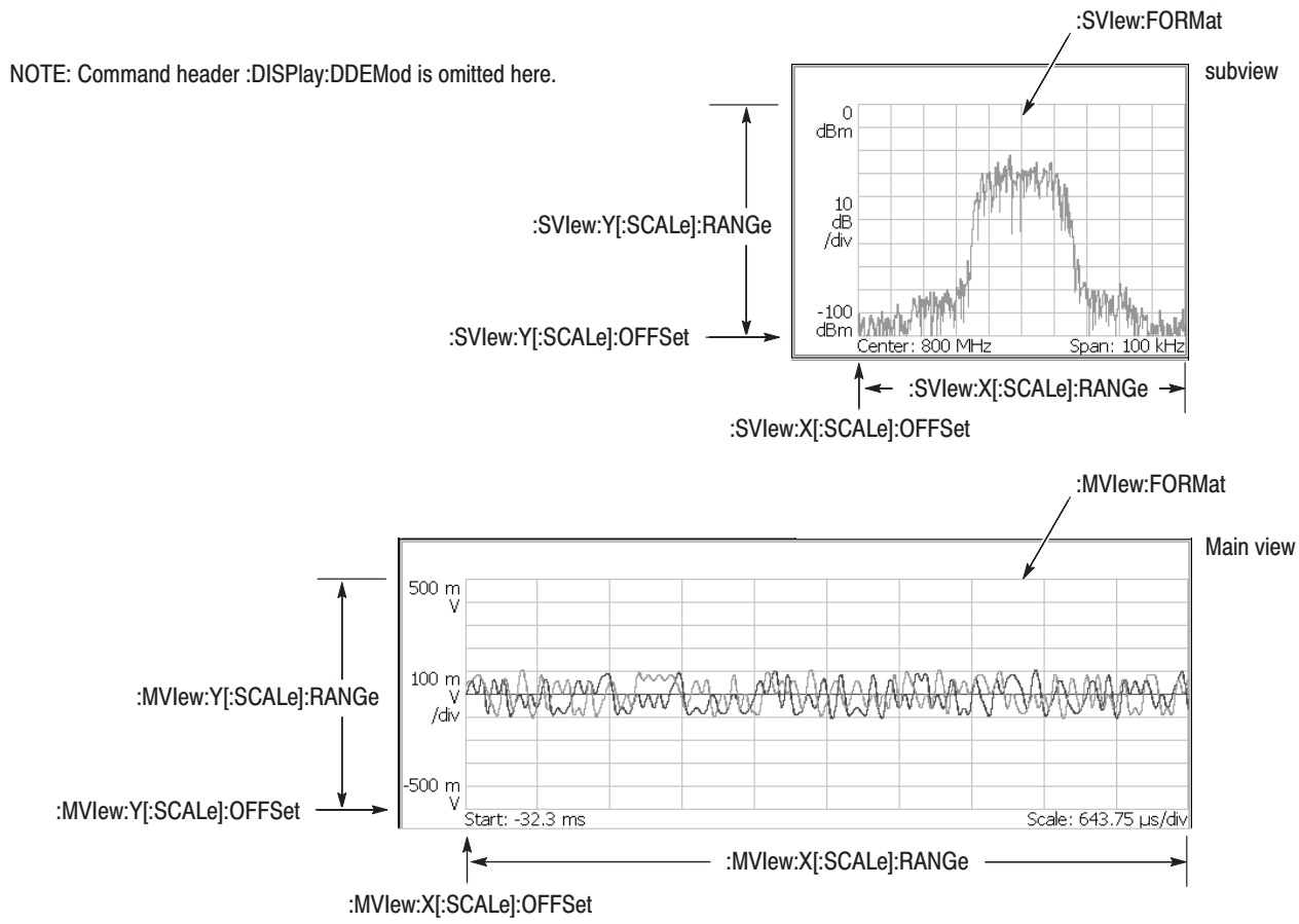
Figure 2-15: :DISPlay:DDEMod command setting
